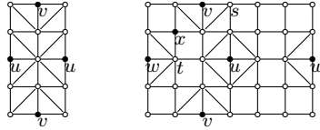
Figure 10: Example and counterexample for Theorem 2.5 of [9]
