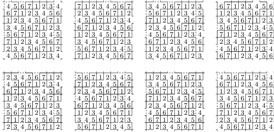
Figure 11: Case r = 3
